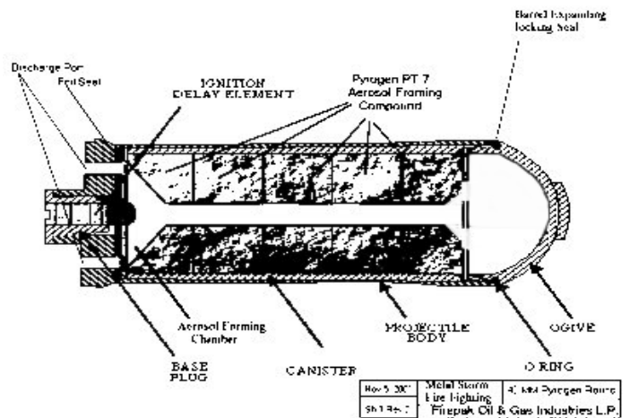
Fig 2. 250g Air Launch PyroGen Generator
